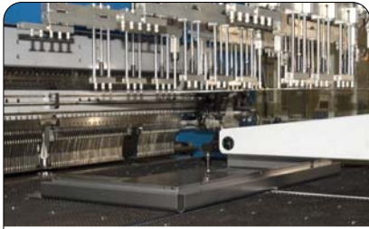
Incorporation of automatic paneling for the automation of the folding process
